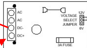
Figure 1: AD12612 Power Supply showing terminal designations and Voltage Select Jumper.
